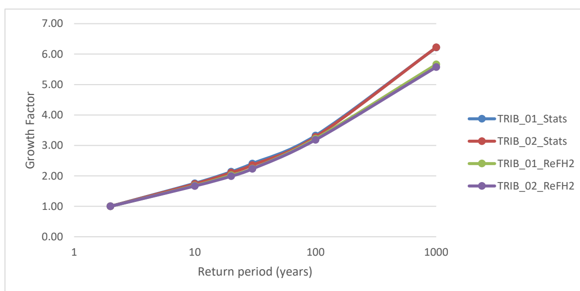
Figure 5-1 Comparison of growth curves between the FEH Statistical and ReFH2 methods
